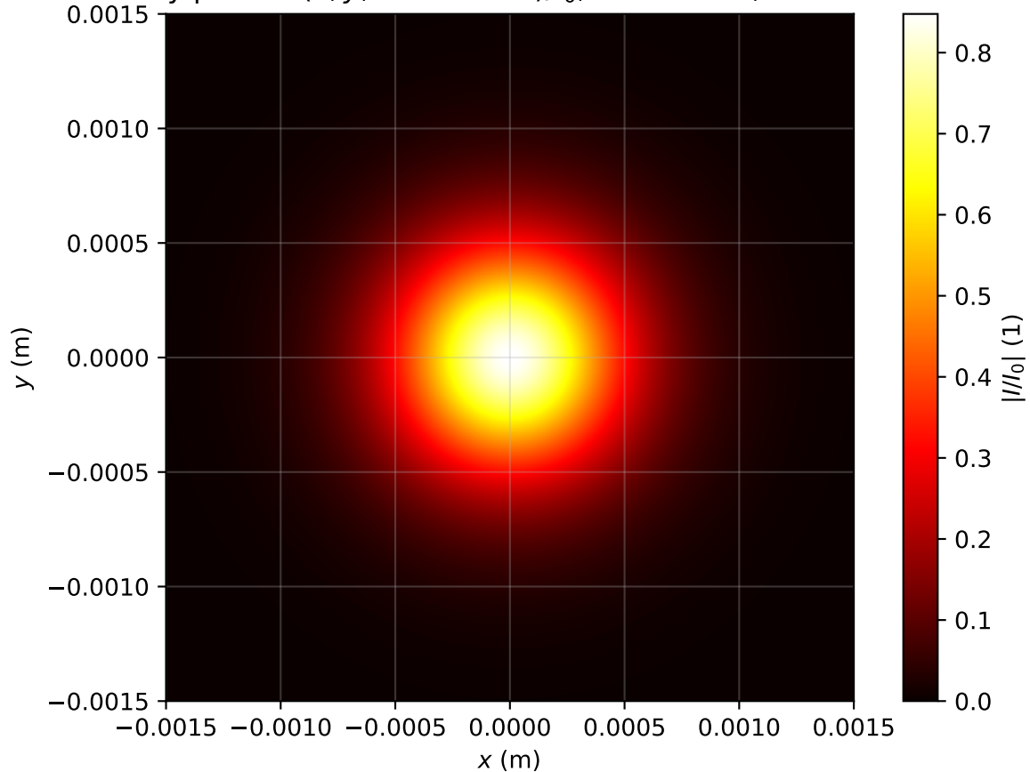
Intensity profile I(x, y, z = 1.911m)/I_0 , \text{Pin}=0.5\text{Pcr} , artificial time
